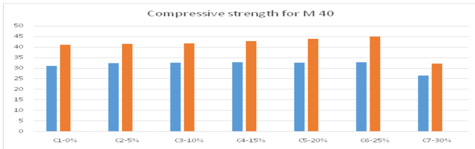
Fig.10. Compressive strength variation for M40grade at 7 & 28days
