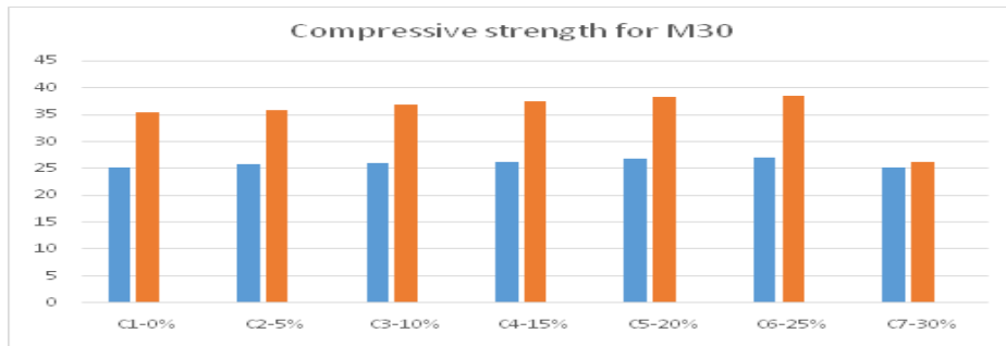
Fig.9. Compressive strength variation for M30grade at 7 & 28days
