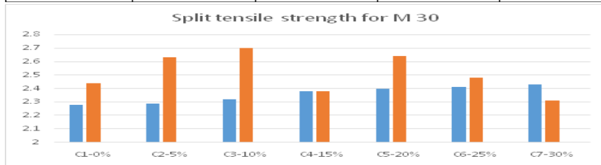
Fig.11. Split tensile strength variation for M30 grade at 7 & 28days
