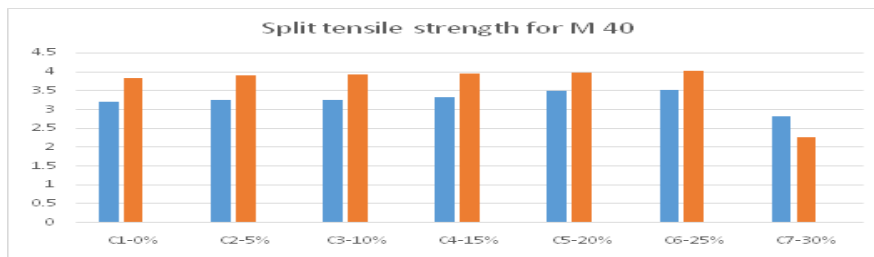
Fig.12.Split tensile strength variation for M40 grade at 7& 28days
